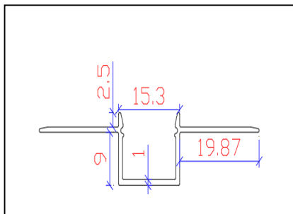
Recessed CL-TX423A
