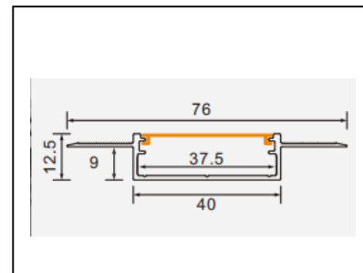
Recessed CL-7609A
